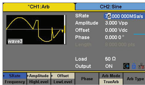
Custom true arbitrary waveform at 75 MSa/s, 8 Mpts
