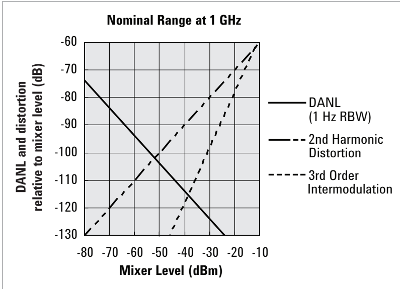
Figure 1. Nominal dynamic range – Band 0, for second and third order distortion, 9 kHz to 3.6 GHz
