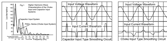
Fig. 2 Input voltage-current curves
