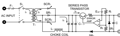
Fig. 5 Basic Circuitry of the PAD-L Series
