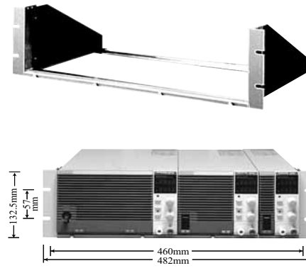
KRA3 Rack Adapter for inch type racks (EIA STANDARD)
