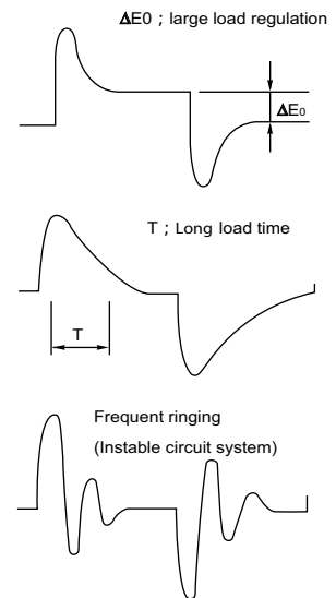
[Fig.-7] Transient Response Waveform
