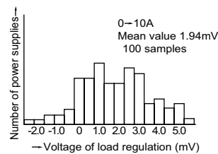
[Fig.-4] Distribution of Load Regulation (CV Characteristics)
