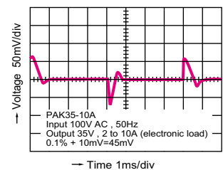
[Fig.-7] Transient Response Waveform
