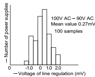
[Fig.-3] Distribution of Line Regulation (CV Characteristics)
