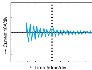
[Fig.-14] Waveform of Rush Current
