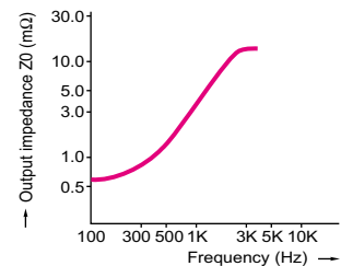
[Fig.-17] Output Impedance Characteristics of PAK35-10A
