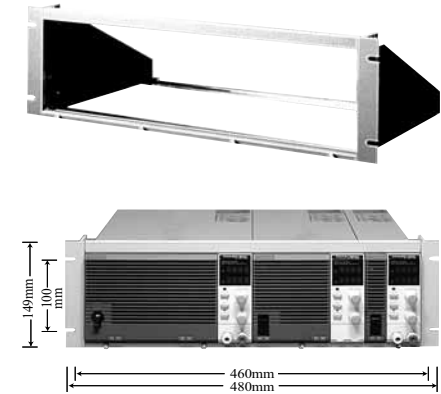
KRA150 Rack Adapter for metric type racks (JIS STANDARD)
