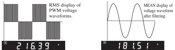
Comparison of voltage display values of RMS and MEAN with the low-pass filter
