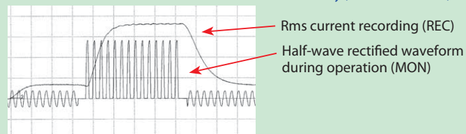
Recording Current Consumption of a Hair Dryer
