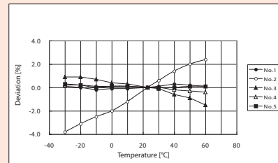
Example of zero-point temperature characteristic (Model 9693 SENSOR)
