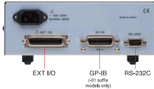
3561-01 Rear Panel
