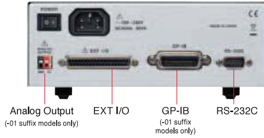
3561-01 Rear Panel
