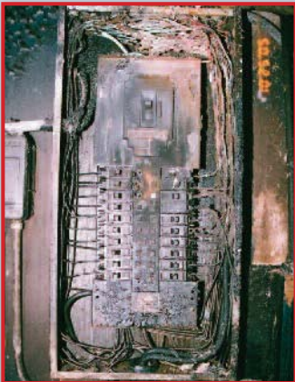
An IRT spot check might have kept this circuit breaker panel from burning out
