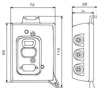
Docking stations
