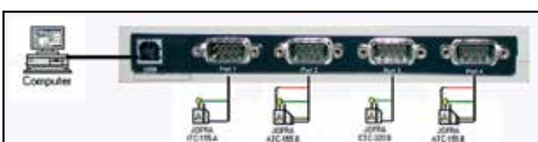
Edgeport converter - Order number 125002 The edgeport converter converts one USB port to four RS232 ports without external power supply. Tested with JOFRA calibrators and JOFRACAL calibration software
