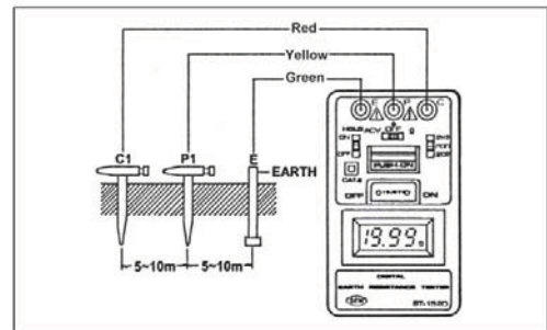
Earth Resistance Measurement
