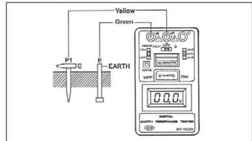
Earth Resistance Measurement
