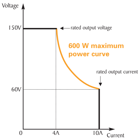
Model 9206 output characteristics
