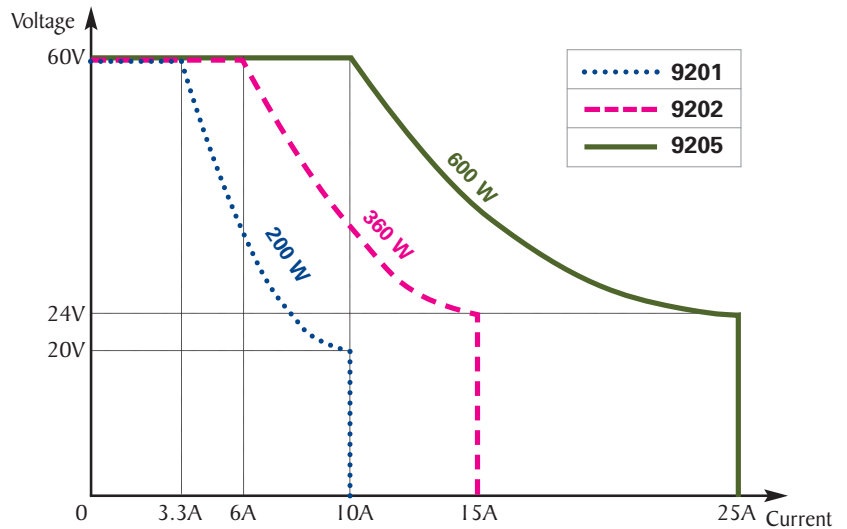
Models 9201 / 9202 / 9205 output characteristics
