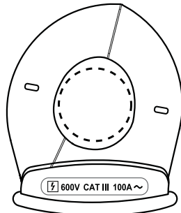
Jaw Opening: 1.10" (28mm) Conductor Size: 1" (26mm)
