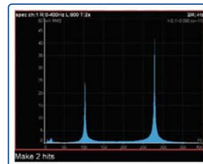
BUMP TEST
