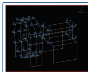
ADS › Animated deflection shapes
