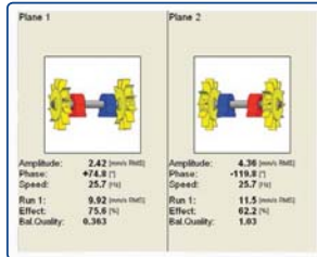
BALANCER › Intuitive graphical balancing procedure
