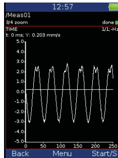
Time signal
