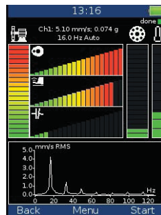
Expert system
