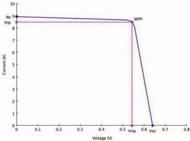
PV simulation curve
